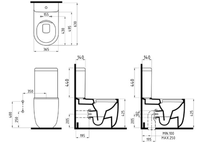
DUVARA SIFIR KLOZET MDKD063N1VS1W5S20 630x365 mm
