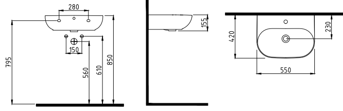
DUVAR MONTAJLI LAVABO BATARYA DELİKLİ / TAŞMA DELİKLİ MDLS05501FD1W5000 550x420 mm
