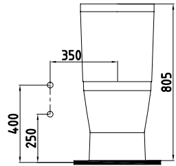
DUVARA SIFIR KLOZET NPKD06301VS1W5SZ0 630x355 mm
