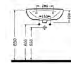
BEDENSEL ENGELLİLER İÇİN LAVABO TPLE06001VD1W3000 600x510 mm
