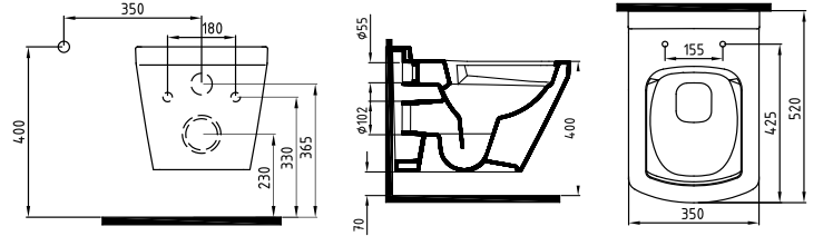
N1 NO-RİM ASMA KLOZET NPKA052N1VP1W5000 520x350 mm
