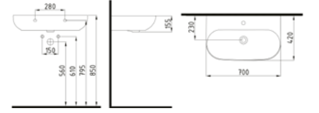
DUVAR MONTAJLI LAVA- BO BATARYA DELİKLİ / TAŞMA DELİKLİ MDLS07001FD1W5000 700x420 mm
