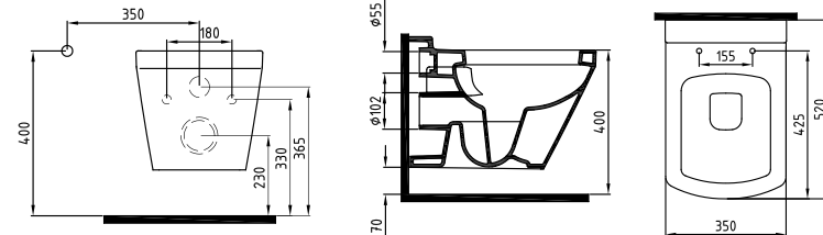
ASMA KLOZET 52 cm TAHARET BORULU NPKA052AMVP1W5000 520x350 mm
